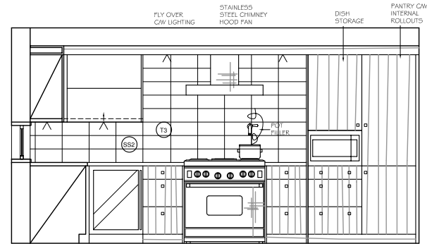
B ELEVATION WINE COOLER WOLF GAS RANGE MICROWAVE CW STAINLESS STEEL FRAMING KIT POT DRAWERS PANTRY CW INTERNAL ROLLOUTS
